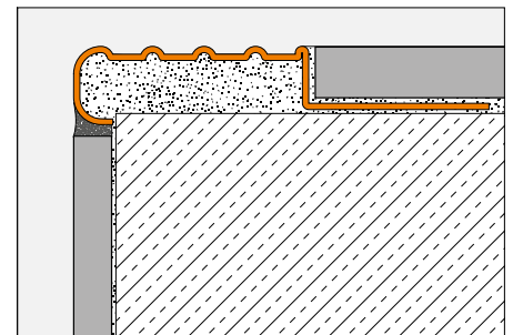
Inbouwvariant Schlüter®-TREP-E
