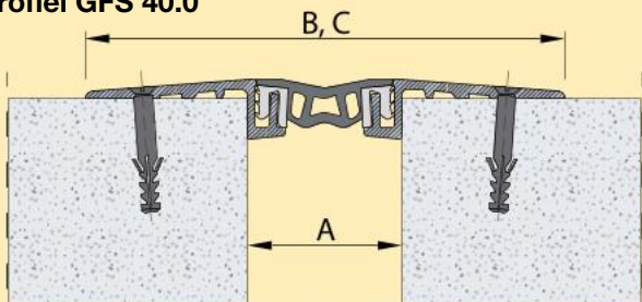
Profiel GFS 40.0
